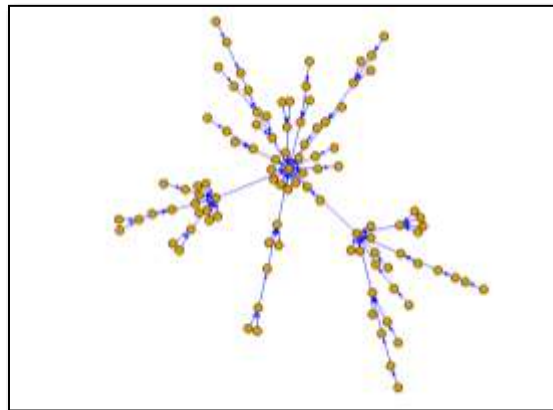
Figure 5. Scale-free network (N=100)
